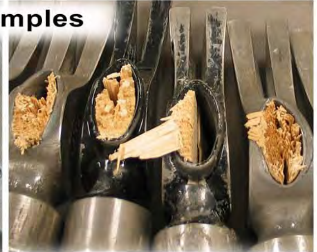
Good grain structure; fibers jagged, Hdl. material pulled down out of eye. Break caused by user over-prying. Not covered by Warranty.
